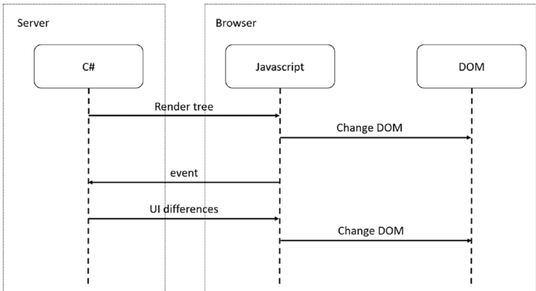
Figure 5. Blazor Server-Side
